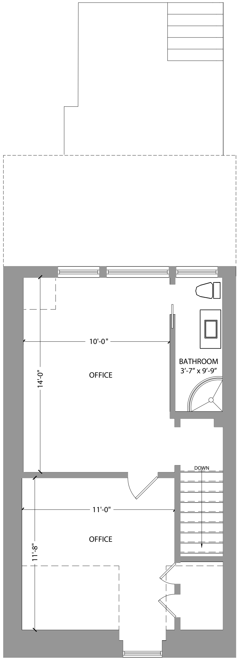
UPPER FLOOR PLAN
